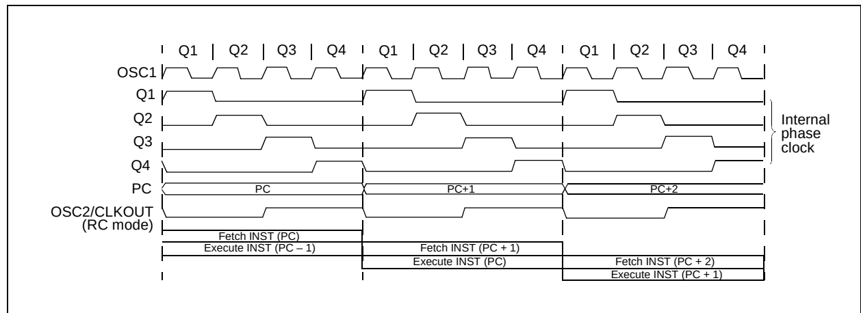
FIGURE 2-2: CLOCK/INSTRUCTION CYCLE
