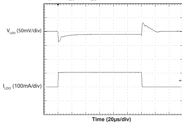
LDO Load Transient Response (1.8V)
