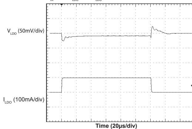
LDO Load Transient Response (1.2V)
