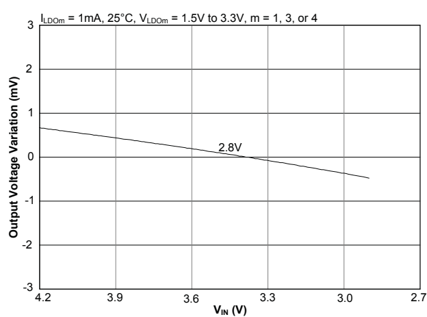
Line Regulation (LDOm)
