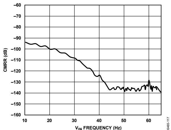
Figure 17. Common-Mode Rejection Ratio (CMRR) vs. V_{IN} Frequency ( V_{IN} = 0.1 V, 10 Hz to 70 Hz, Output)
