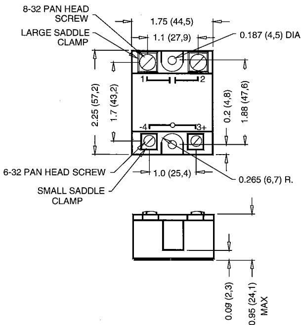
DIMENSIONS: INCHES (MILLIMETERS) TOLERANCE: \pm 0.020 ( \pm 0.50 )
