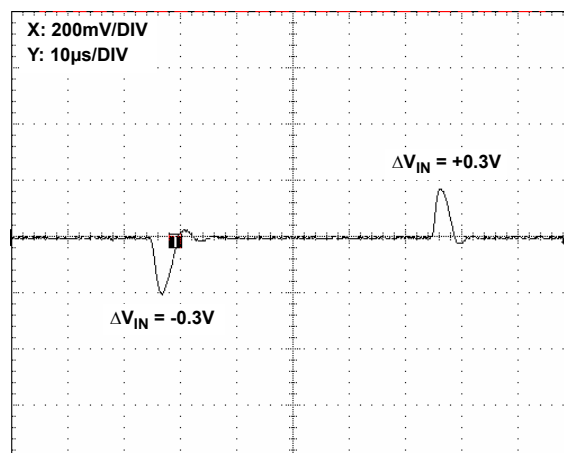
FIGURE 22. LINE TRANSIENT RESPONSE, NO CAPACITIVE LOAD
