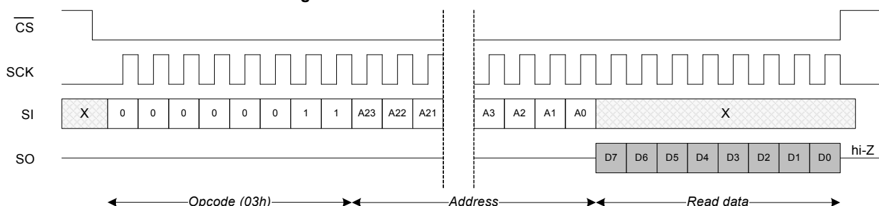
Figure 19. READ Instruction in SPI Mode
