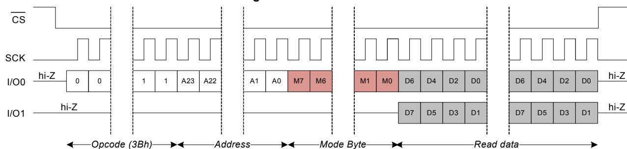
Figure 26. DOR Instruction
