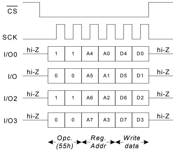
Figure 52. WRTC Instruction in QPI Mode
