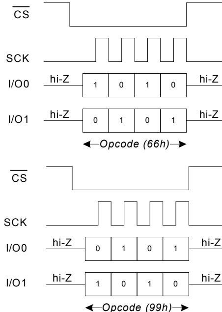
Figure 41. RESET Instruction in DPI Mode
