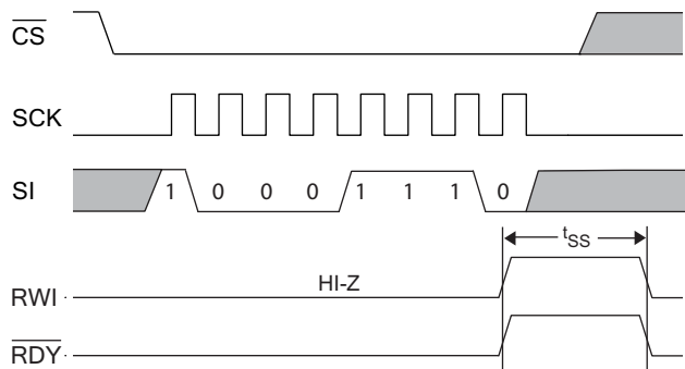
Figure 109. AutoStore Enable Cycle
