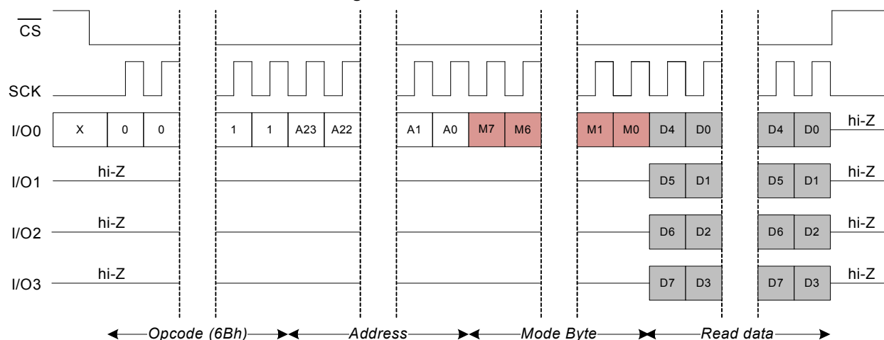
Figure 27. QOR Instruction
