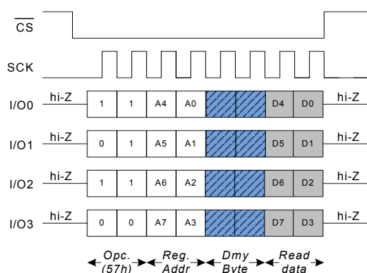
Figure 49. FAST_RDRTC Instruction in QPI Mode
