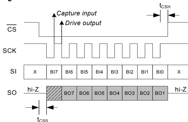
Figure 5. SPI Mode 3
