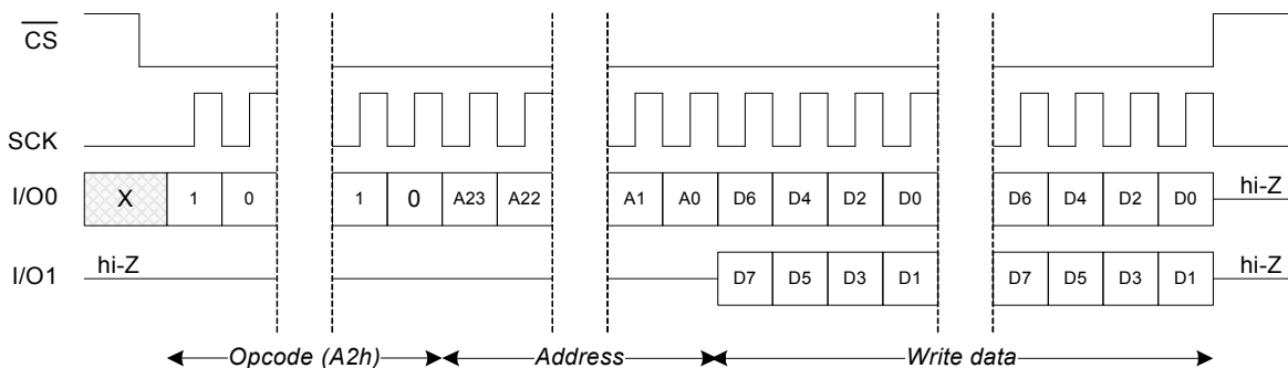
Figure 34. DIW Instruction
