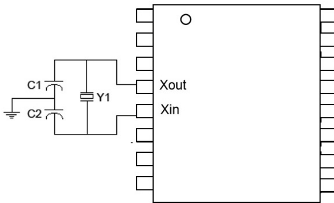
Figure 102. RTC Recommended Component Configuration [1]
