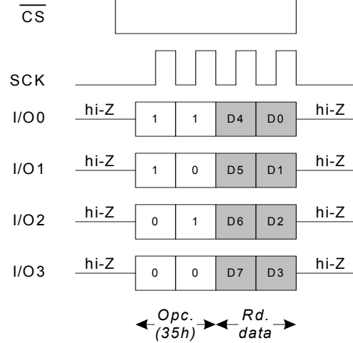
Figure 70. RDCR Instruction in QPI Mode
