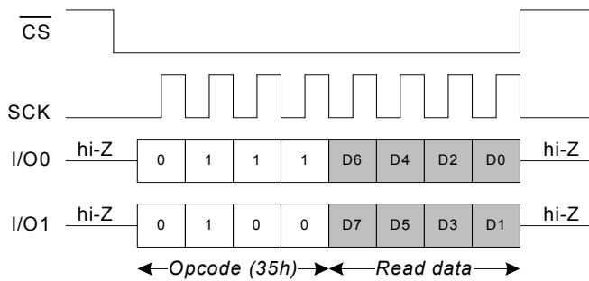
Figure 69. RDCR Instruction in DPI Mode
