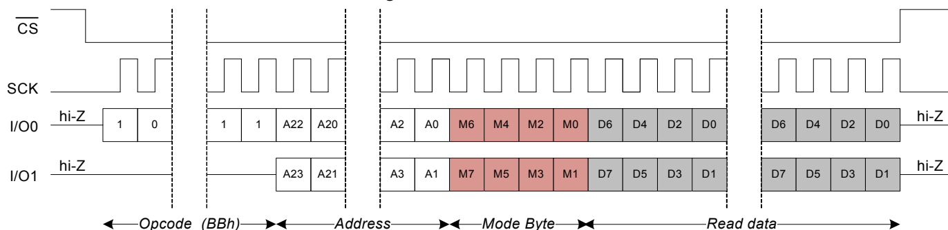
Figure 28. DIOR Instruction
