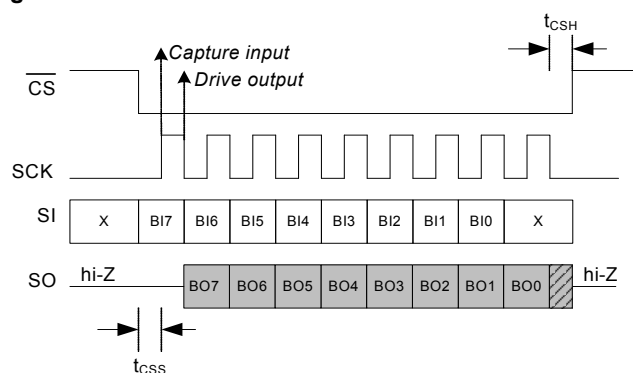
Figure 4. SPI Mode 0
