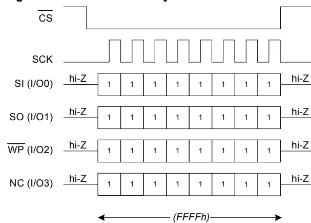
Figure 43. Default Recovery Instruction
