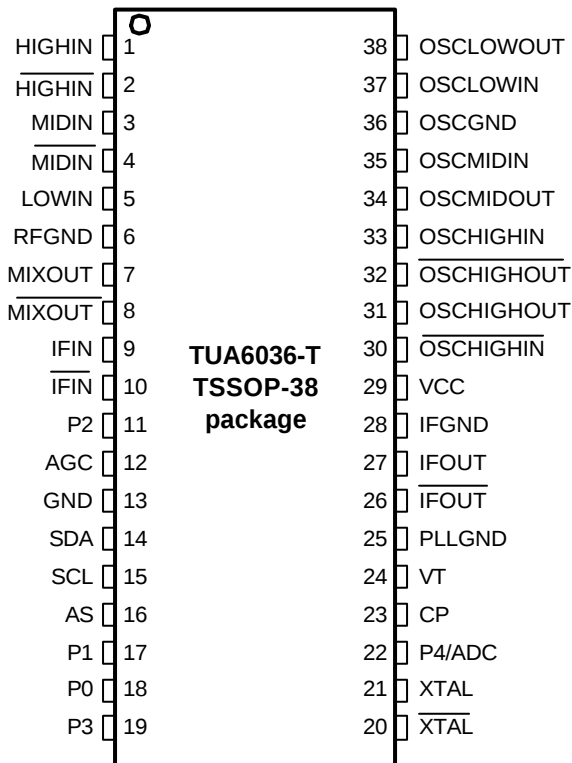
Figure 2 Pin Configuration TUA6036 in TSSOP-38 Package
