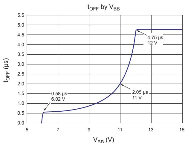
Figure 3. When V_{BB} falls below 12 V, t_{OFF} decreases
