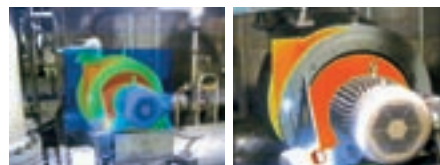
Alpha Blending
