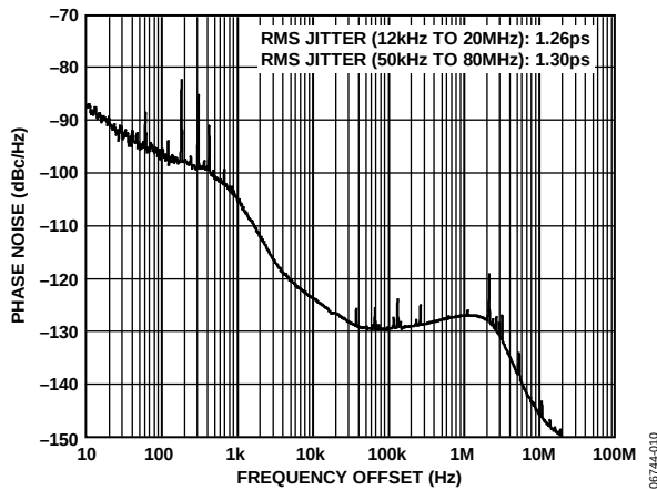
Figure 10. Additive Phase Noise at HSTL Output Driver, SYSCCLK = 1 \text{ GHz} ( SYSCCLK \text{ PLL Enabled and Driven by a } 25 \text{ MHz Fox Crystal Oscillator} ), f_{REF} = 19.44 \text{ MHz} , f_{OUT} = 155.52 \text{ MHz} , DPLL \text{ Loop BW} = 1 \text{ kHz}
