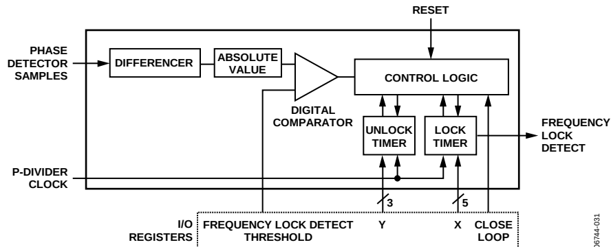
Figure 30. Frequency Lock Detection
