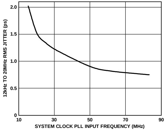
Figure 9. 12 kHz to 20 MHz RMS Jitter vs. System Clock PLL Input Frequency, SYSCCLK = 1 \text{ GHz} , f_{REF} = 19.44 \text{ MHz} , f_{OUT} = 155.52 \text{ MHz}
