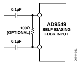
Figure 21. FDBK_IN Input
