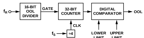
Figure 32. Reference Monitor
