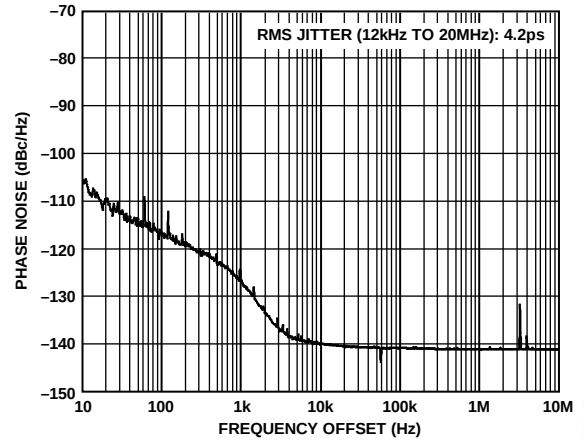
Figure 11. Additive Phase Noise at HSTL Output Driver, SYSCCLK = 500 \text{ MHz} ( SYSCCLK \text{ PLL Disabled} ), f_{REF} = 10.24 \text{ MHz} , f_{OUT} = 20.48 \text{ MHz} , DPLL \text{ Loop BW} = 1 \text{ kHz}
