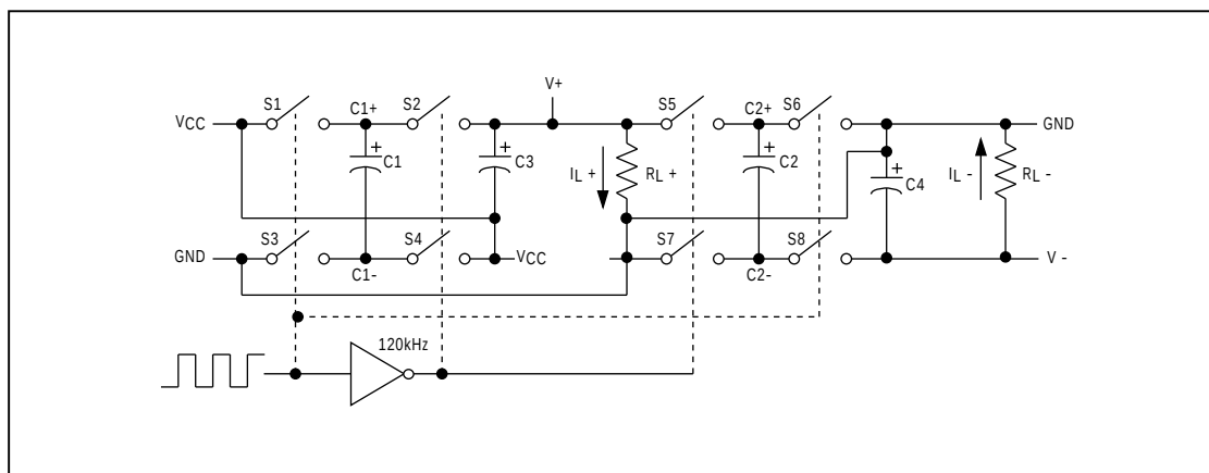
Figure 2. Charge-Pump Diagram
