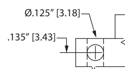
SIDE MOUNTING (S)
