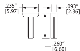
PLM-K2 KEY IN CONTACT (ORDER SEPARATELY)
