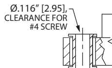
FLOATING BOBBIN (F)
