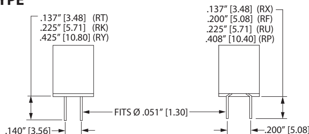
NARROW DIP SOLDER (RT, RK, RY)
