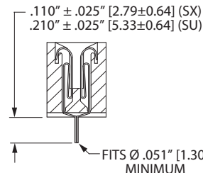
CENTERED DIP SOLDER (SX, SU) AVAILABLE WITH DUAL OR HALF LOADED READOUT TYPE
