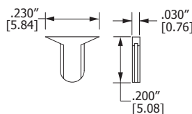
PLA-K1 KEY IN BETWEEN CONTACTS (ORDER SEPARATELY)
