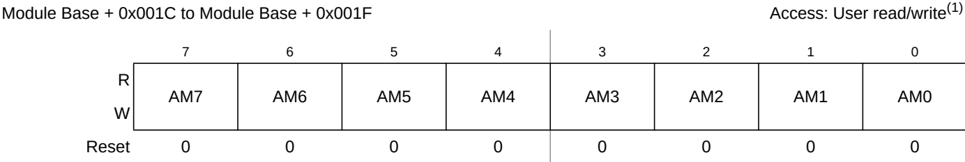
Figure 8-23. MSCAN Identifier Mask Registers (Second Bank) — CANIDMR4–CANIDMR7
