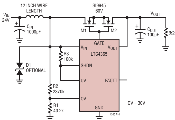
Figure 14. 0V Fault with Large V_{IN} Inductance
