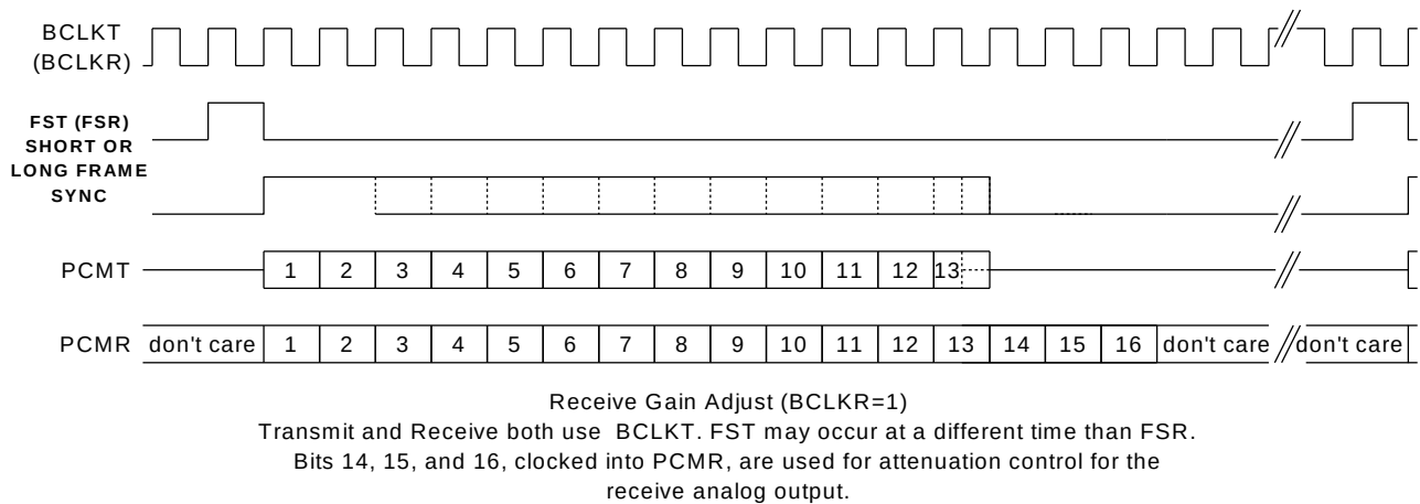
FIGURE 7.7: RECEIVE GAIN ADJUST TIMING MODE
