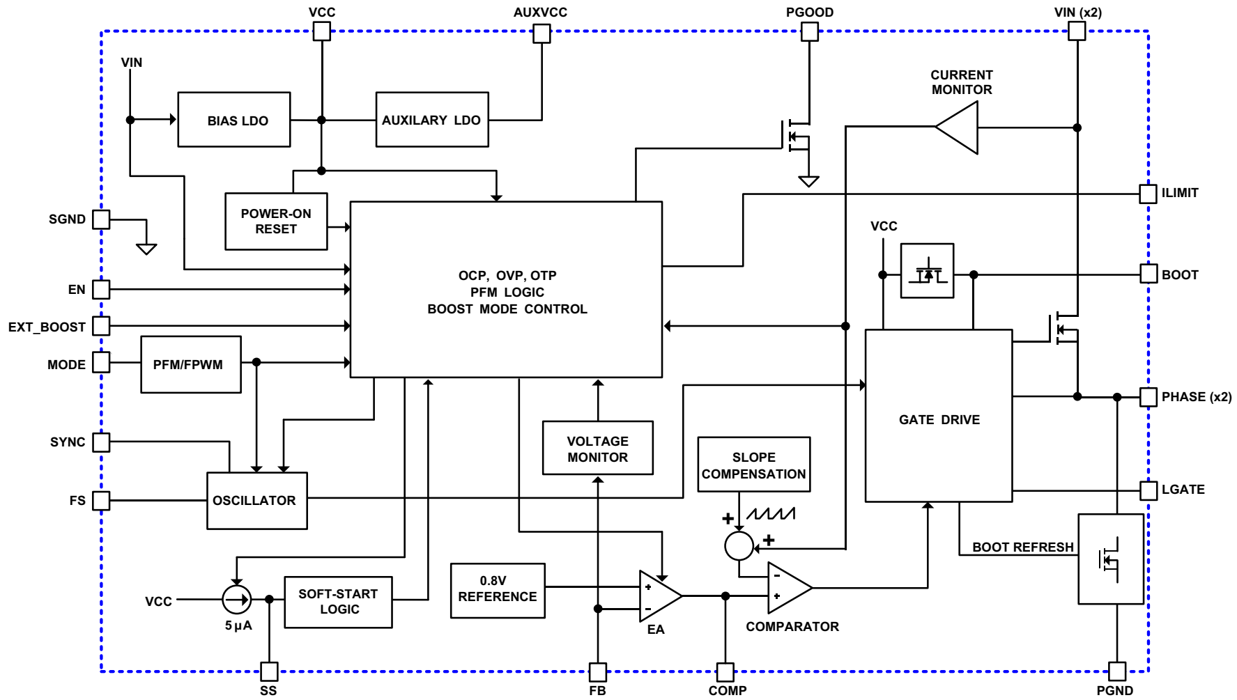
FIGURE 3. BLOCK DIAGRAM
