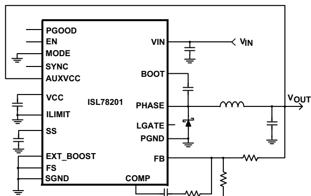
FIGURE 5B. NON-SYNCHRONOUS BUCK
