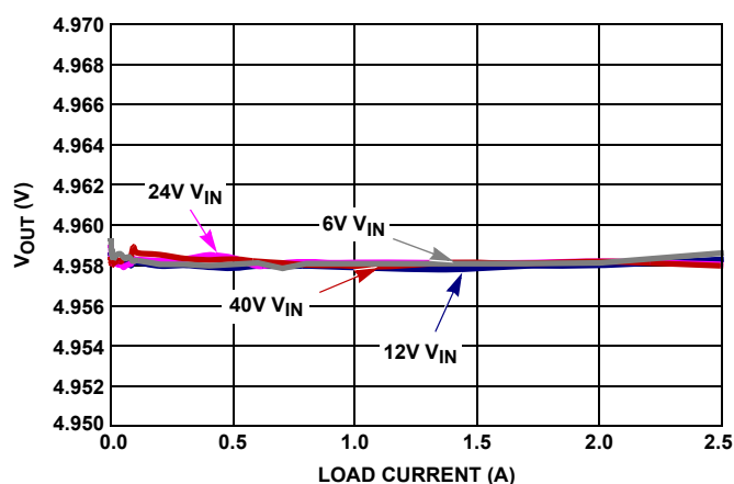
FIGURE 10. LOAD REGULATION, V_{OUT} 5V, T_A = +25^\circ\text{C}
