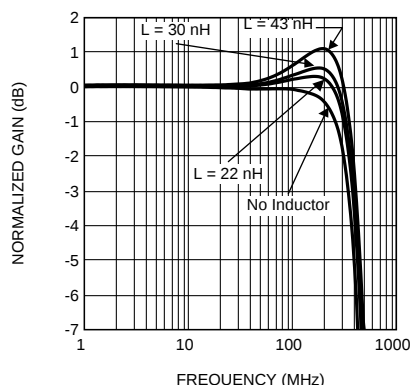
Figure 48. Termination Inductor Bandwidth Enhancement Using Input 0
