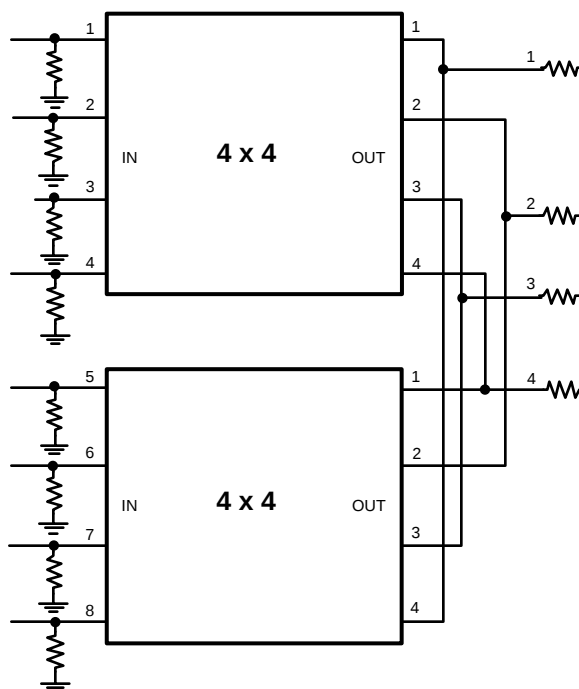
Figure 44. Input Expansion with Shared Termination Resistors (Only 4 input and 4 output channels shown for illustration purposes.)
