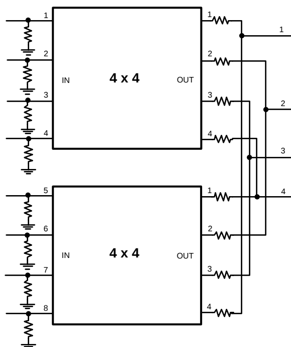
Figure 45. Input Expansion with Separate Termination Resistors (Only 4 input and 4 output channels shown for illustration purposes.)
