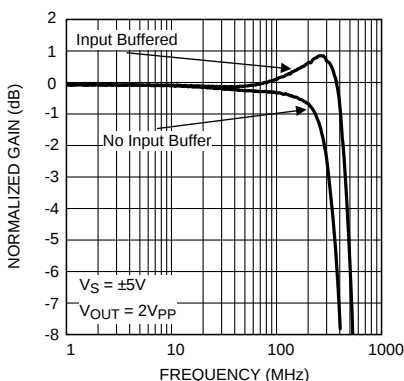
Figure 42. Frequency Response for Buffered and Unbuffered Output expansion
