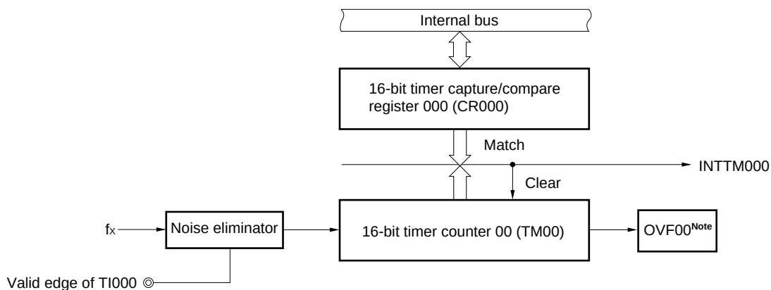
Figure 6-27. Configuration Diagram of External Event Counter
