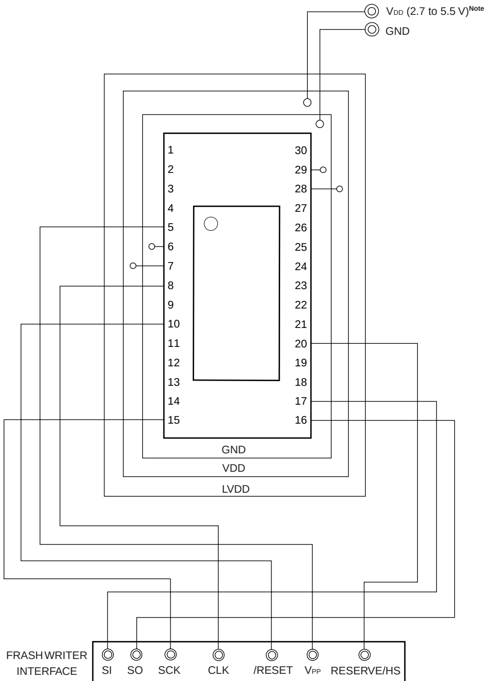
Figure 21-3. Example of Wiring Adapter for Flash Memory Writing in 3-Wire Serial I/O (CS10 + HS) Mode
