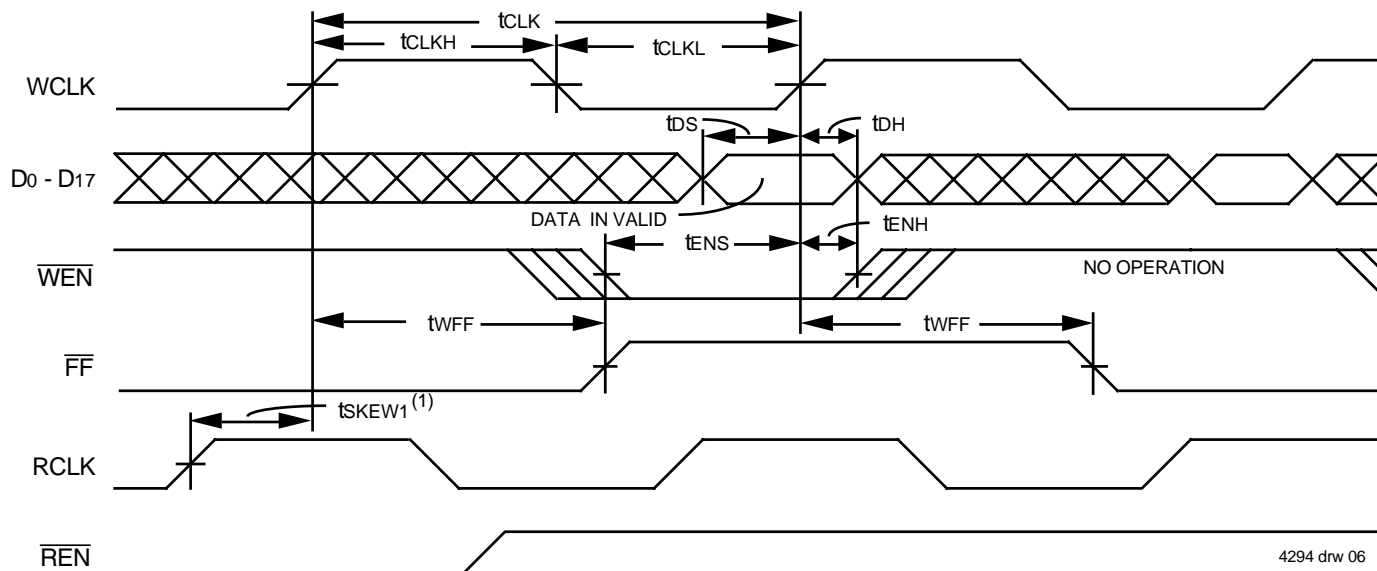
Figure 5. Reset Timing (2)
