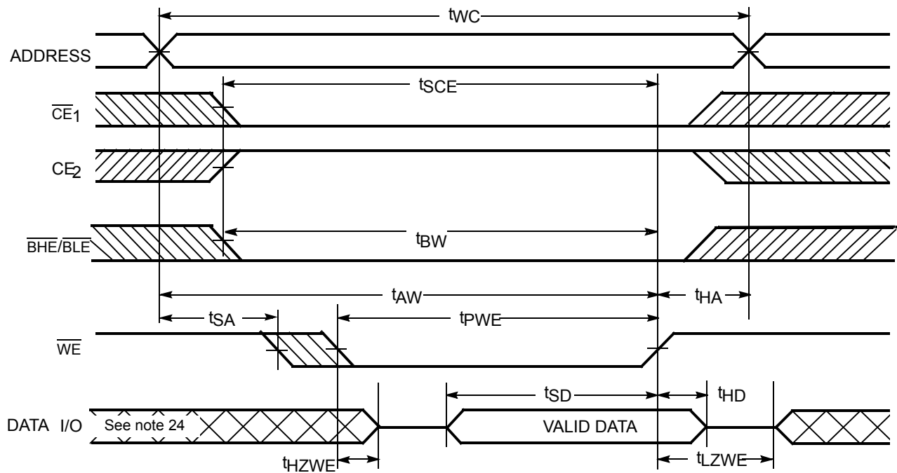
Write Cycle 3 ( \overline{\text{WE}} Controlled, \overline{\text{OE}} LOW) [24, 25]
